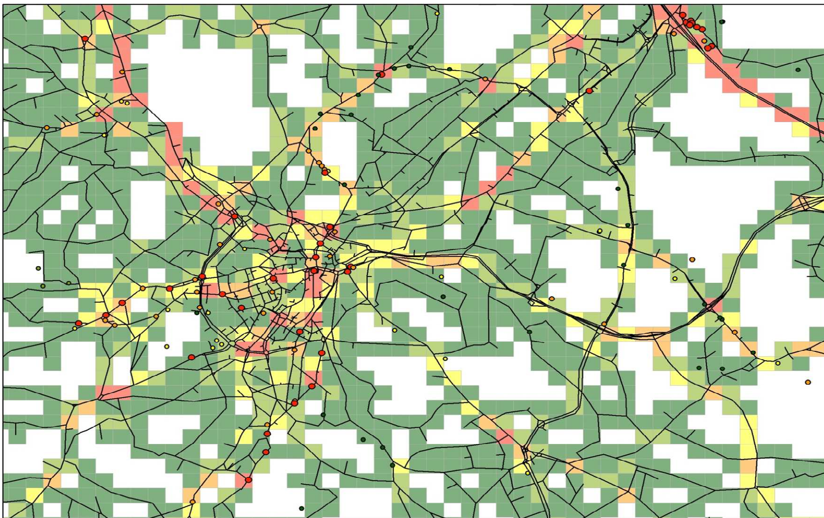
Figure G1 Comparison of Observed NO x Air Quality at 2011 and Modelled NO x Emissions at 2015
