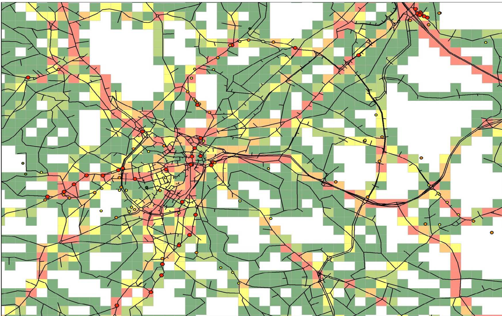
Figure F3 Comparison of Observed NO x Air Quality at 2008 and Modelled NO x Emissions at 2008
