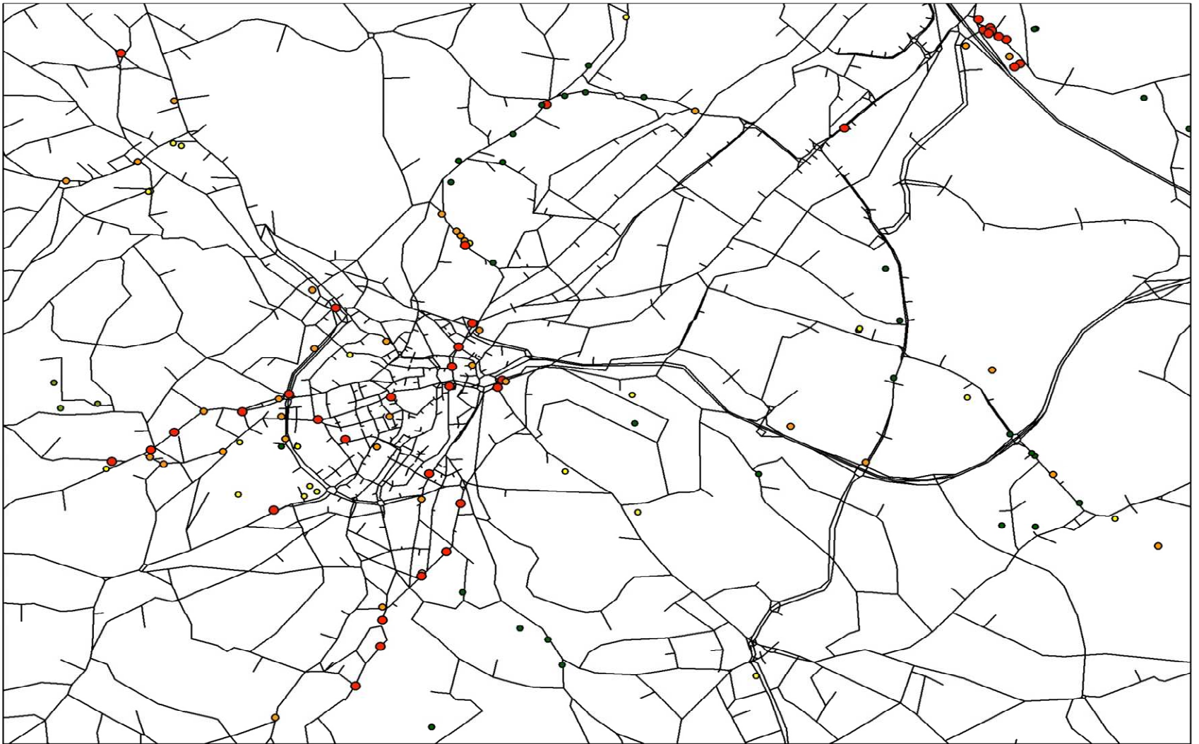
Figure F2 Observed Air Quality at 2011
