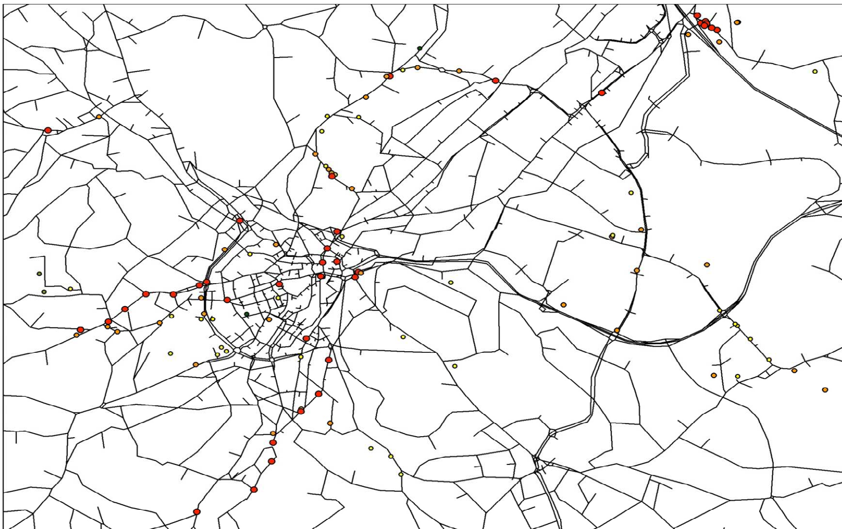
Figure F1 Observed Air Quality at 2008
